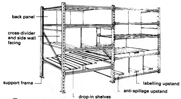
4 Wide-span racking (depth 600-1100mm)
